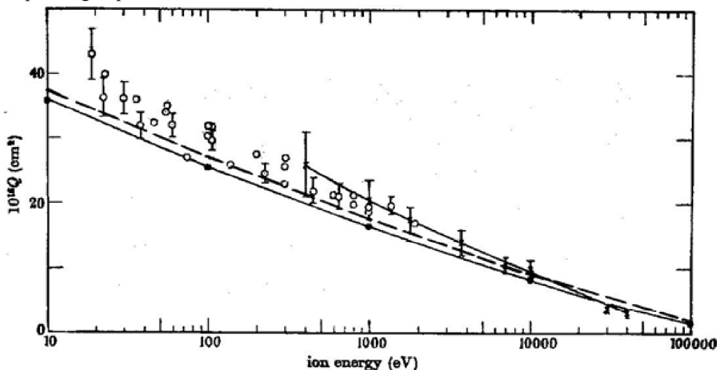
Fig. 1. Comparison of the experimental cross-sections of the resonant charge exchange between hydrogen atoms and low energy protons with the corresponding theoretical cross-sections (the cross-sections are in units of 10^{-16} cm 2 ). Circles (some with error margins) – experiment reported in paper [2]; crosses (with error margins) connected by the solid line – experiment reported in paper [1]; filled circles connected by the solid line – theory from paper [13], allowing only for the usual hydrogen atoms; the dashed line – theory from the present paper, allowing for the SFHA.
