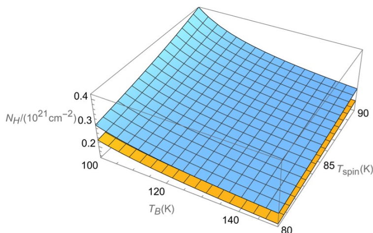
Fig. 1. Dependence of the column density N_H on the spin temperature T_{\text{spin}} of the usual hydrogen atoms and on the brightness temperature T_B for two scenarios. The upper surface corresponds to the neglect of the SFHA. The lower surface corresponds to the allowance for the SFHA.
