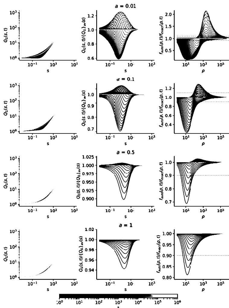
Figure 1. The result of accuracy analysis of automodel solution for various values of the Voigt parameter and the propagation front \rho = \rho_r taken in the form (25), for different values of t in the range from t_{\min} = 30 to t_{\max} = 10^6 : (left) functions Q_{G2}(s, t) (29); (center) normalized functions Q_{G2}(s, t) / \{Q_{G2}\}_{av}(s) , where subscript av denotes averaging over time from t_{\min} = 30 to t_{\max} = 10^6 ; (right) relative errors of the automodel solution f_{\text{auto}}(\rho, t) / f_{\text{exact}}(\rho, t) .
