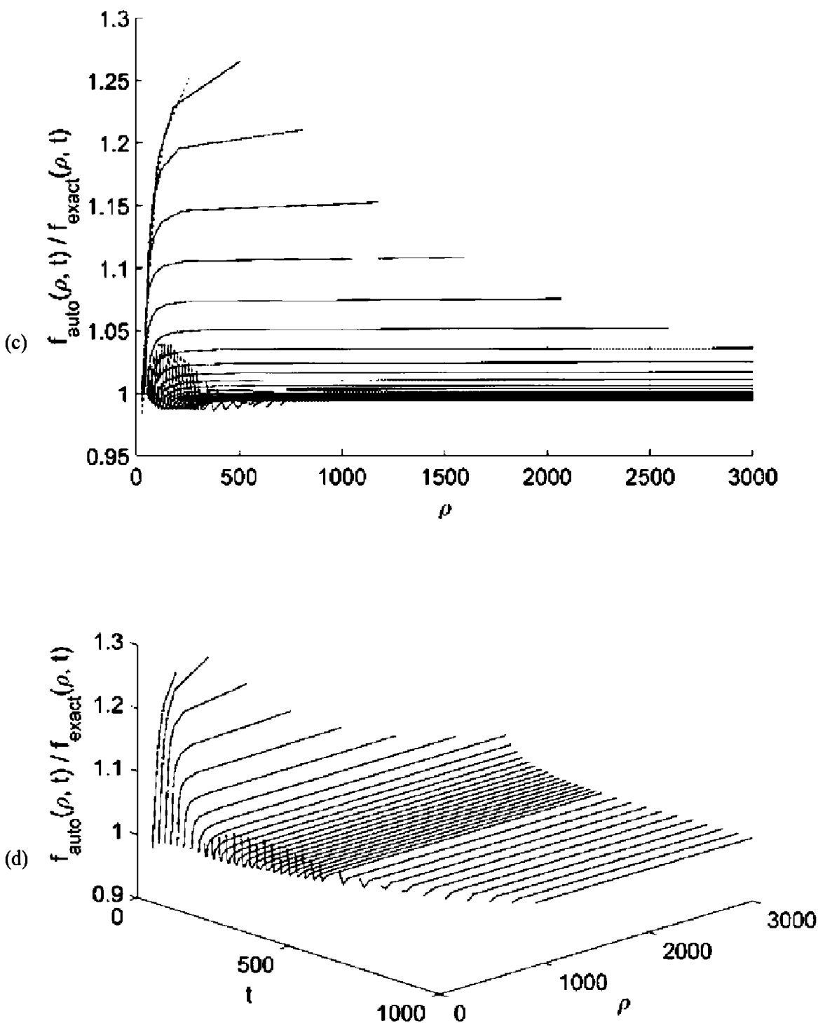
Figure 3. The result of accuracy analysis of automodel solution for the propagation front \rho = \rho_r taken in the form (24), for different values of t in the range from t_{\min} = 40 (dashed line in (a) and (c) subplots and extreme left line in (b) and (d) subplots) to t_{\max} = 10^3 (extreme right line in (b) and (d) subplots) with the time step equal to 20, if 40 \leq t \leq 500 , and 50; if 500 < t \leq 1000 : (a) functions Q_{G2}(s, t) (29); (b) normalized functions Q_{G2}(s, t) / \{Q_{G2}\}^*(s, t) , where \{Q_{G2}\}^*(s, t) is equal to Q_{G2}(s, t = 160) , for small s , and Q_{G2}(s, t = 10^3) , for large s ; (c) relative error of the automodel solution f_{\text{auto}}(\rho, t) / f_{\text{exact}}(\rho, t) , (d) the same in the 3D view.
